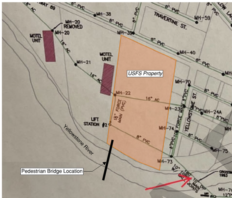
Figure 3. Utilities in vicinity of USFS property
