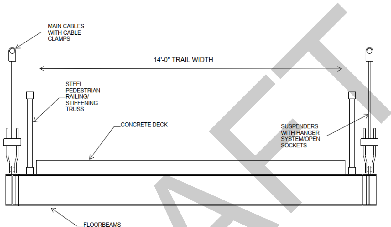
Figure 13: Traditional Steel Deck Arch Cross Section
