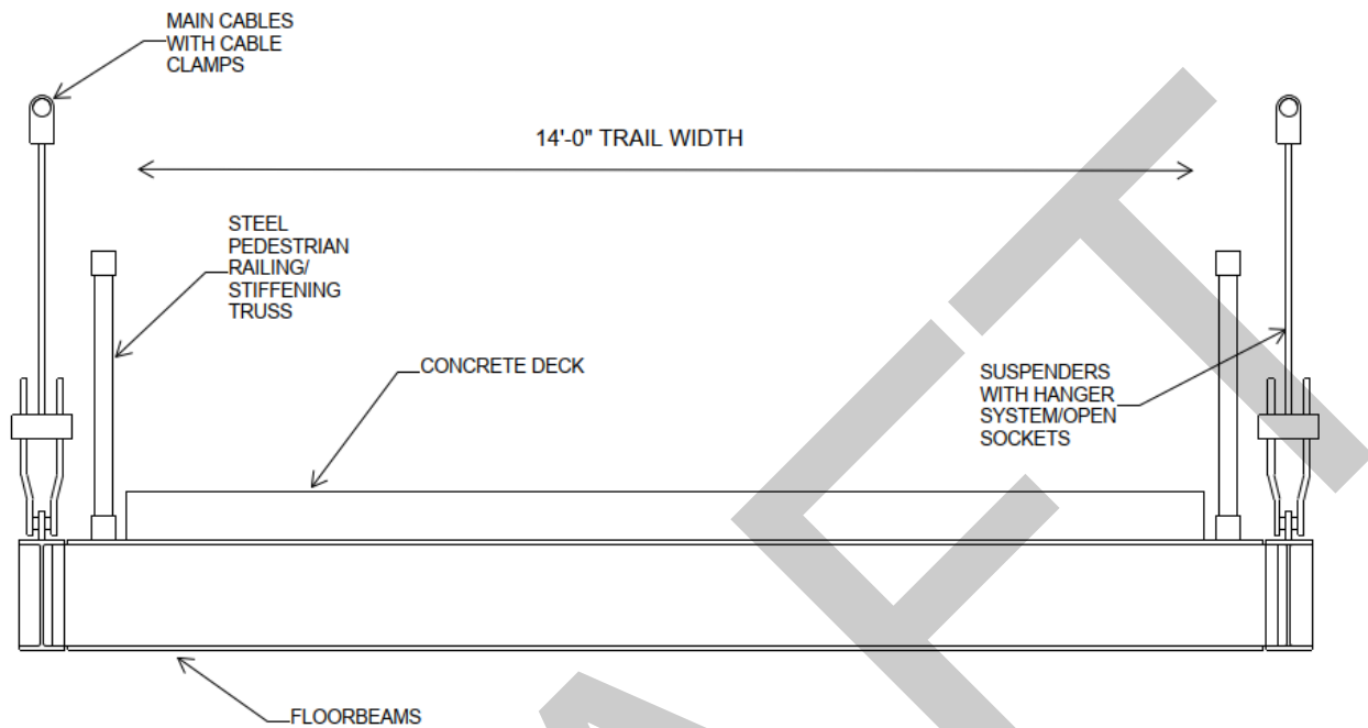
Figure 16: Suspension Bridge Cross Section
